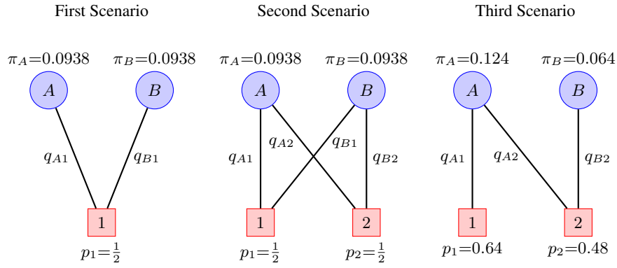
Fig. 1. This figure represents the three scenarios of our example. Vector \mathbf{q} = (\frac{1}{4}, \frac{1}{4}) represents the unique equilibrium in the first scenario. Vector \mathbf{q} = (\frac{1}{8}, \frac{1}{8}, \frac{1}{8}, \frac{1}{8}) is the unique equilibrium of the second scenario. Finally, Vector \mathbf{q} = (0.18, 0.1, 0.16) is the unique equilibrium in the third scenario.
